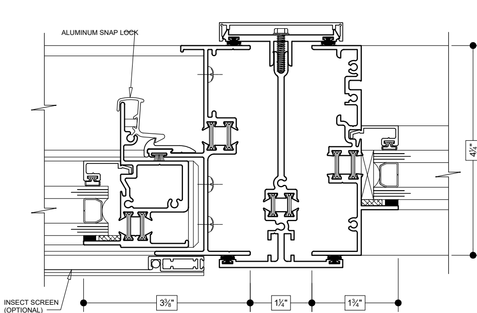
3-PIECE MULLION (HORIZONTAL SLIDING TO FIXED)
