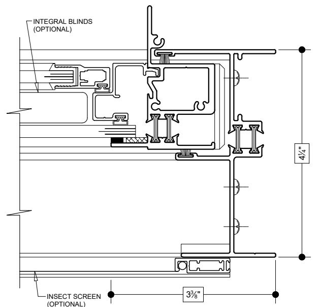
(29) RIGHT JAMB (HORIZONTAL SLIDING)
