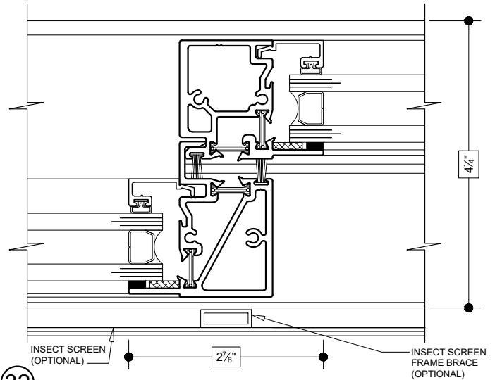
32 MEETING RAIL (HORIZONTAL SLIDING-FIXED SASH TO HORIZONTAL SLIDING)
