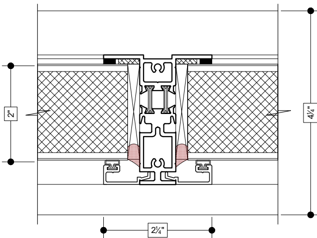
30 TRUE MUNTIN (FIXED PANEL TO FIXED PANEL)
