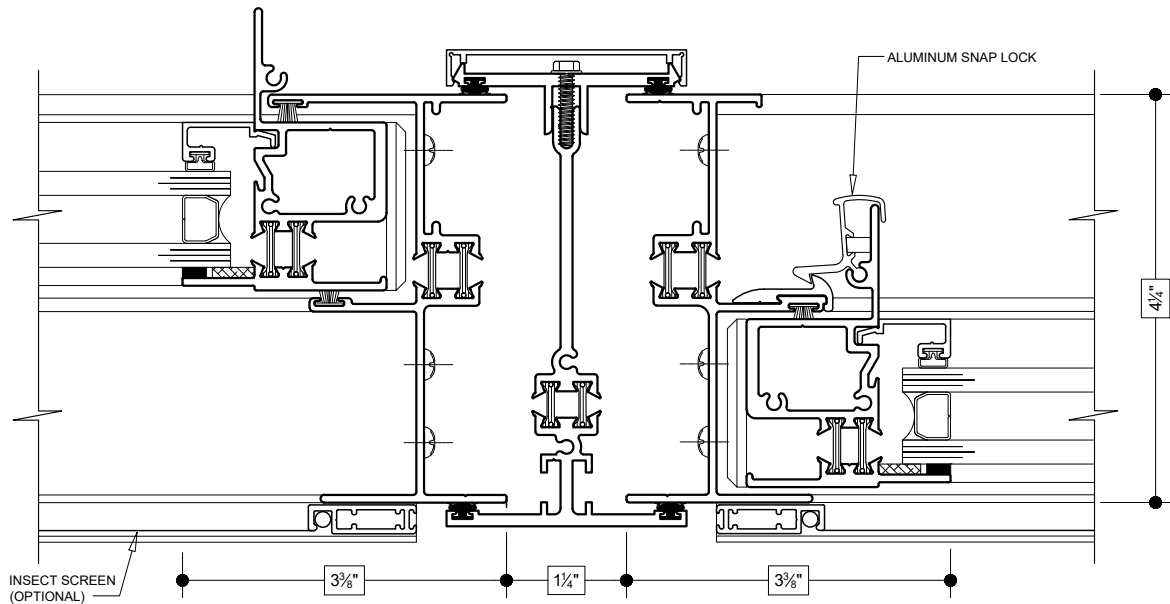
3-PIECE MULLION (HORIZONTAL SLIDING TO HORIZONTAL SLIDING)
