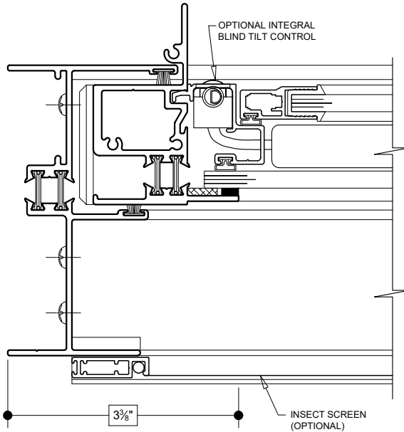
(26) LEFT JAMB (HORIZONTAL SLIDING)
