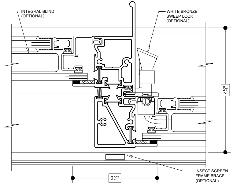
(28) MEETING RAIL (HORIZONTAL SLIDING TO HORIZONTAL SLIDING-FIXED SASH)
