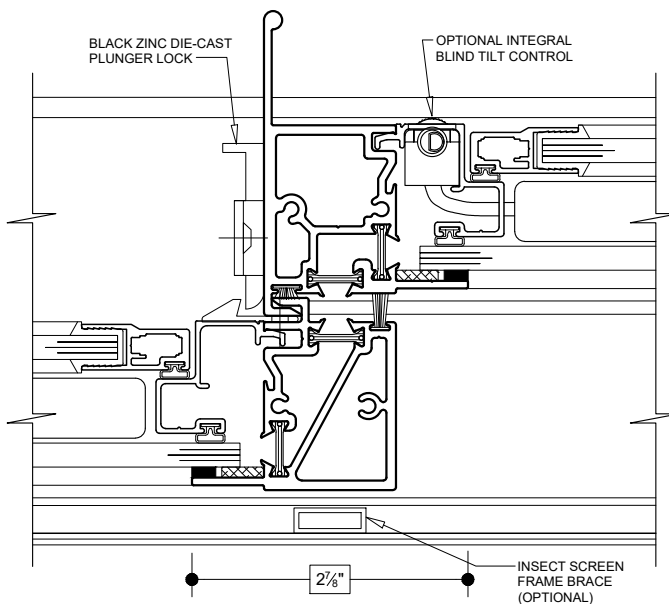
(27) MEETING RAIL (HORIZONTAL SLIDING-FIXED SASH TO HORIZONTAL SLIDING)
