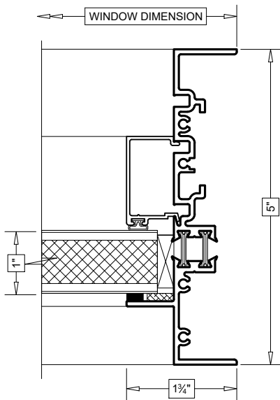
18 3-PIECE MULLION (FIXED PANEL TO FIXED PANEL)
