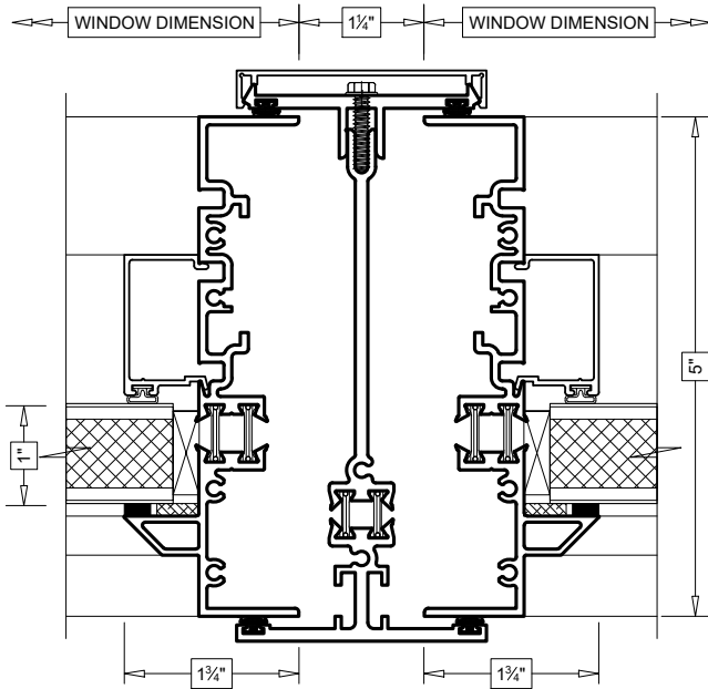
18 3-PIECE MULLION (FIXED PANEL TO FIXED PANEL)
