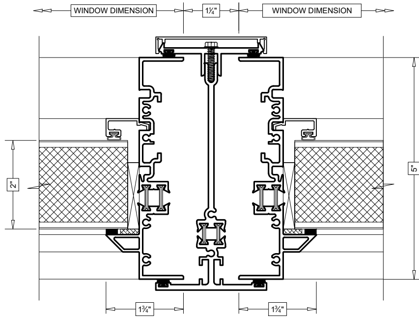
28 3-PIECE MULLION (FIXED PANEL TO FIXED PANEL)
