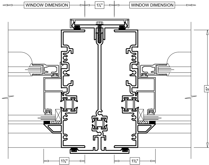
27 3-PIECE MULLION (FIXED TO FIXED)
