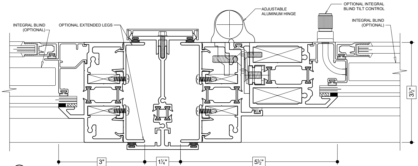
19 3-PIECE MULLION (FIXED TO INSWING)
