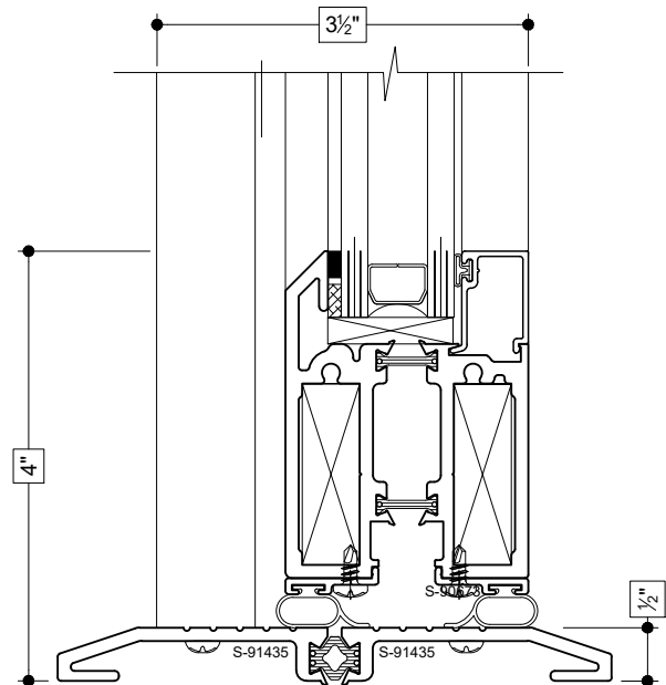
0 PSF SILL (INSWING)
