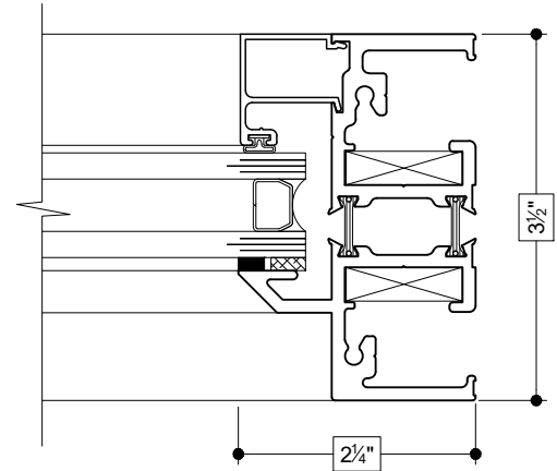
12 RIGHT JAMB (FIXED)
