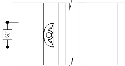
10 APPLIED MUNTIN (COLONIAL)
