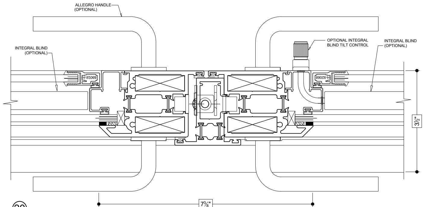
20 INTERMEDIATE (INSWING)
