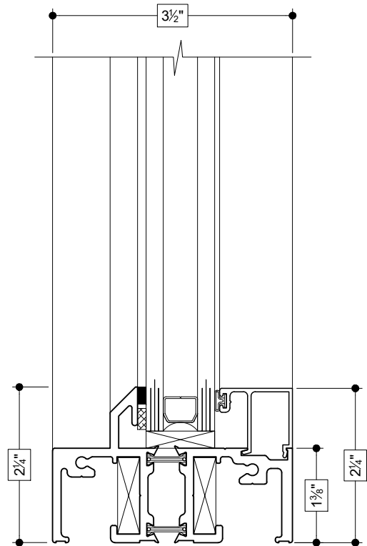
13 SILL (FIXED)
