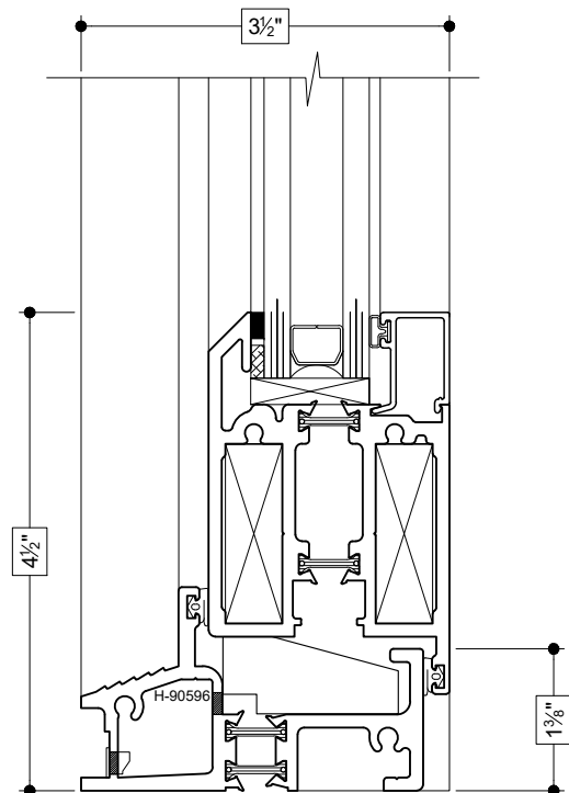
4.5 PSF SILL (INSWING)
