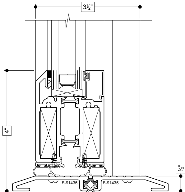
0 PSF SILL (OUTSWING)
