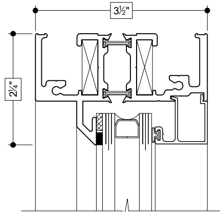
9 HEAD (FIXED)
