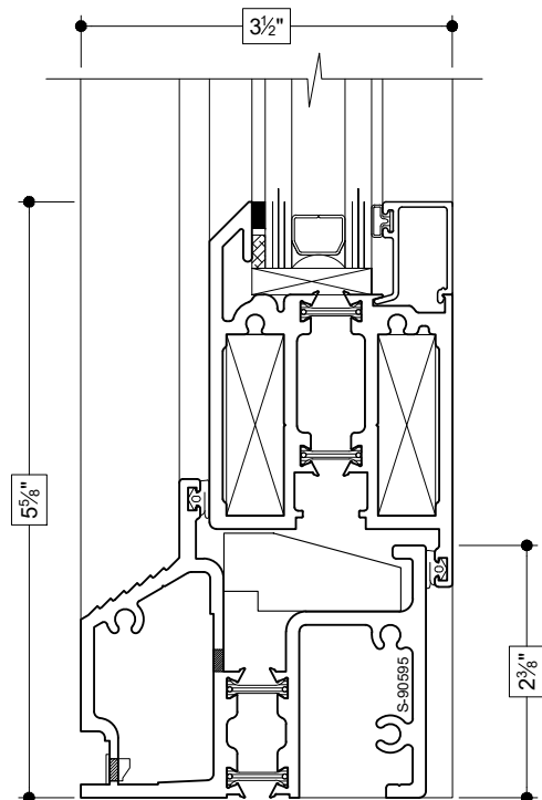
10 PSF SILL (INSWING)
