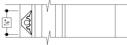
10 APPLIED MUNTIN (TRAPEZOIDAL)
