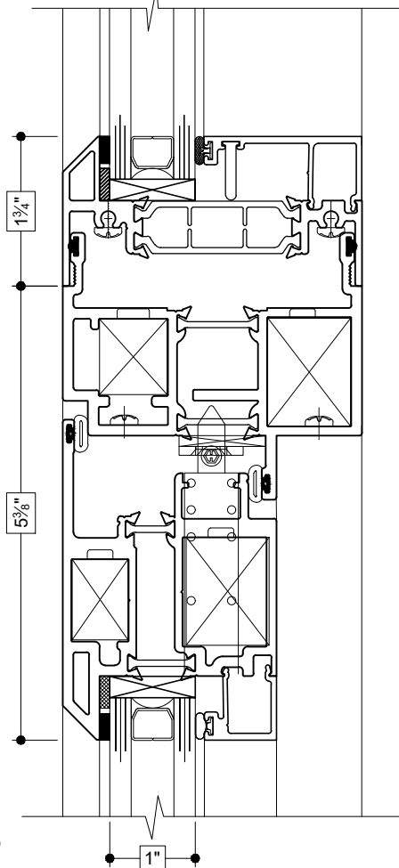
11 SELF-STACK (FIXED OVER OUTSWING)
