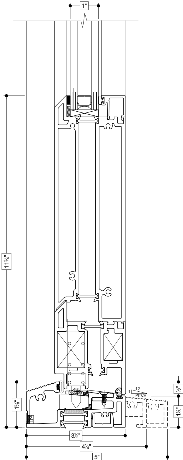
INSWING SILL w/ KICK PLATE
