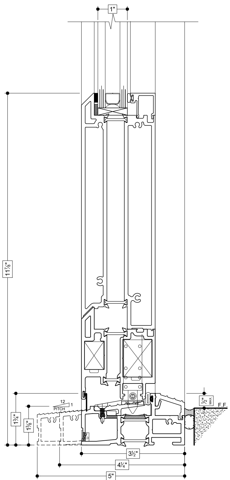
OUTSWING SILL w/ KICK PLATE
