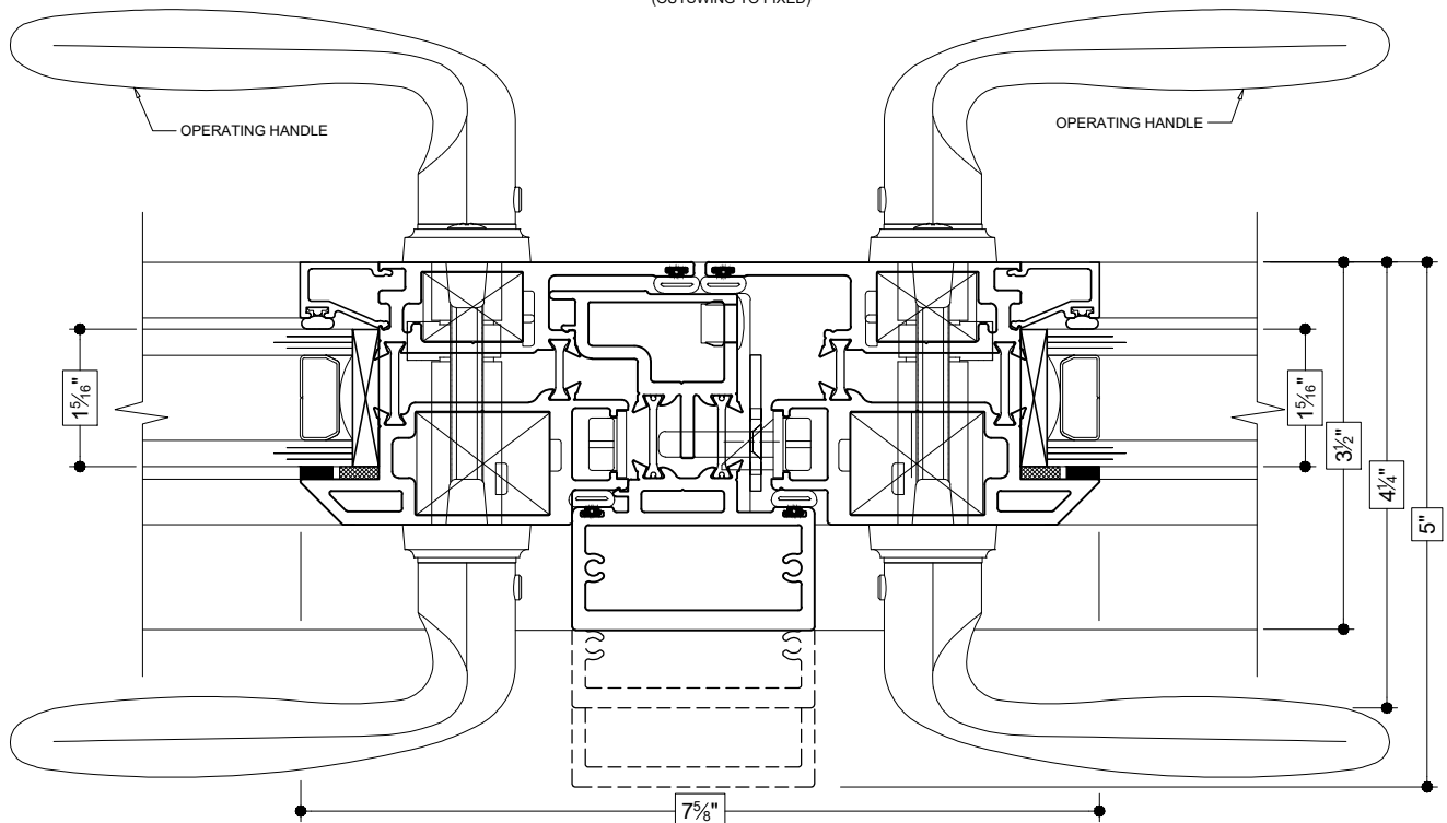
DOOR ADAPTOR (5" DEPTH) (OUTSWING TO FIXED)
