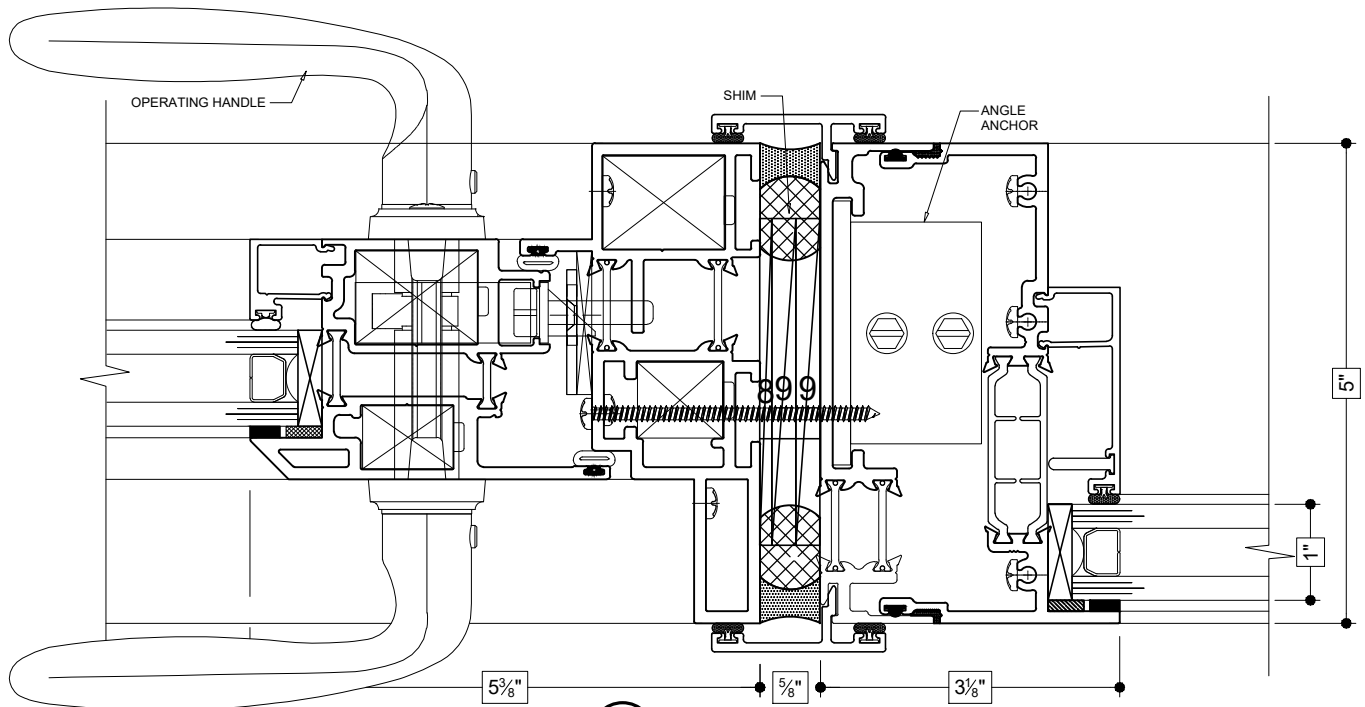
DOOR ADAPTOR (5" DEPTH) (OUTSWING TO FIXED)
