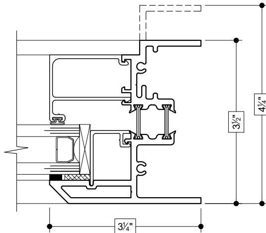
5 RIGHT JAMB (FIXED)
