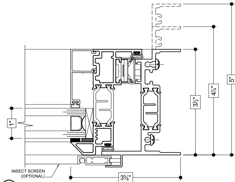
15 RIGHT JAMB (PROJECT-IN - BEVELED FRAME)
