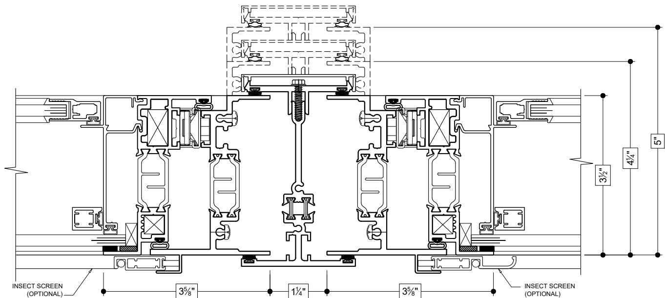
3 PIECE MULLION (PROJECT-IN TO PROJECT-IN)
