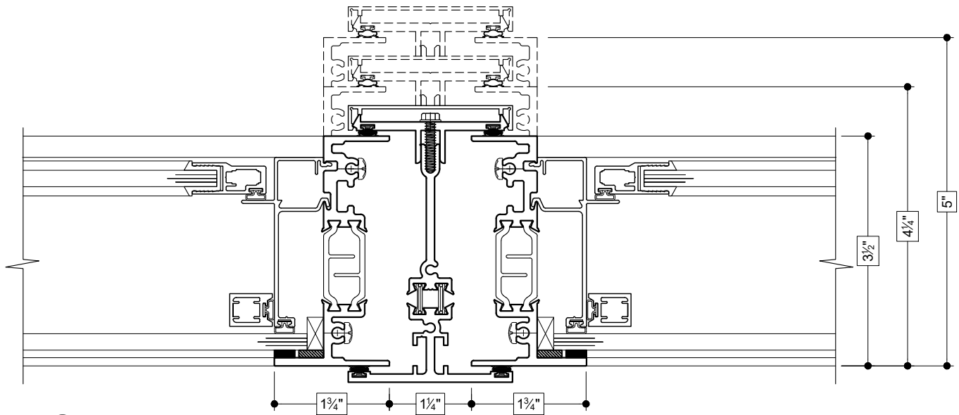
3 PIECE MULLION (FIXED TO FIXED)
