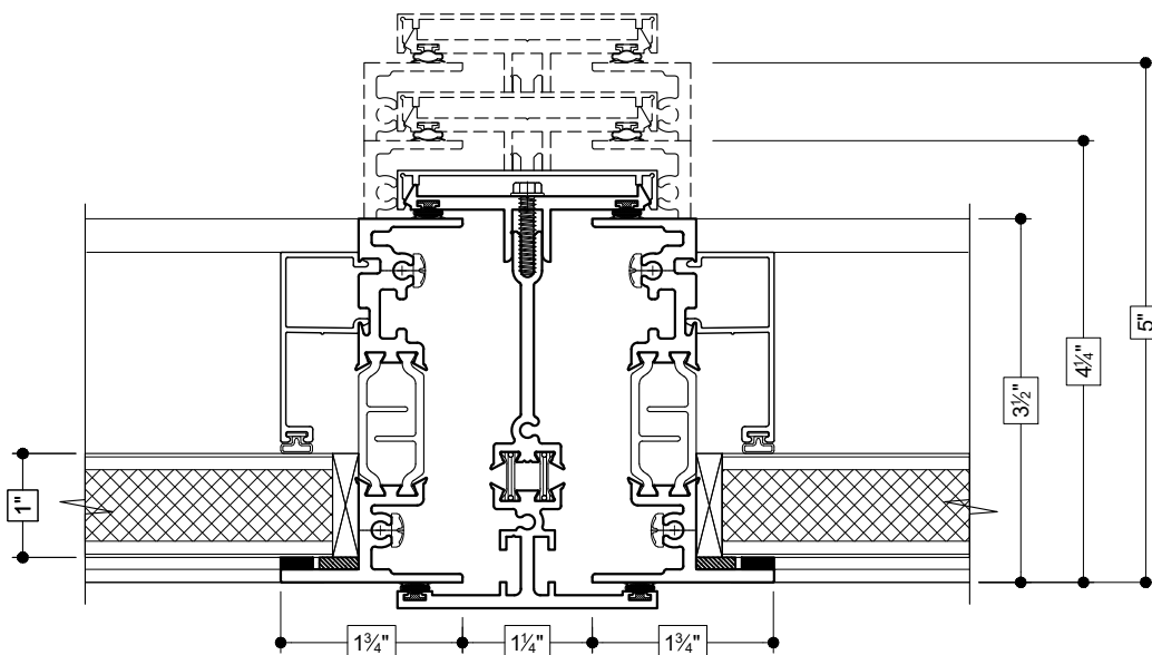
32 3 PIECE MULLION (FIXED PANEL TO FIXED PANEL)
