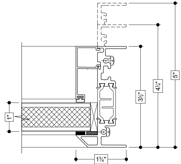
16 RIGHT JAMB (FIXED PANEL - BEVELED FRAME)
