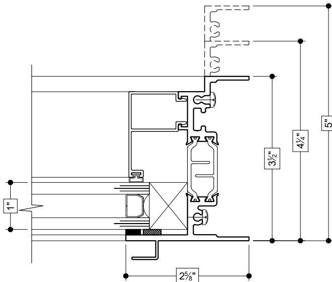
30 RIGHT JAMB - OFFSET (FIXED)
