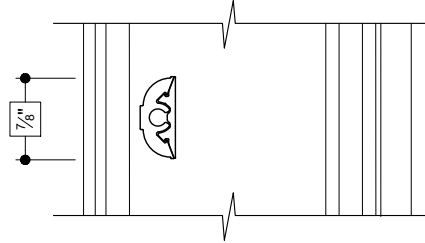
37 INTERNAL MUNTIN (COLONIAL)
