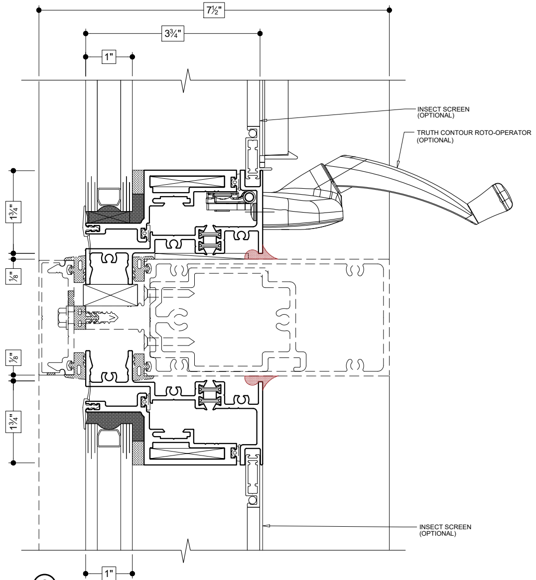
6 SILL & HEAD (PROJECT-OUT OVER PROJECT-OUT)
