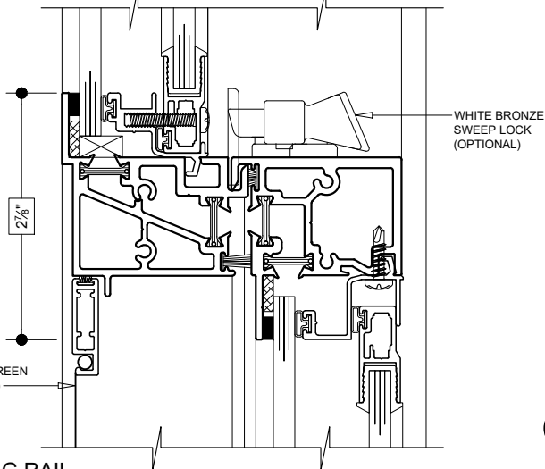
(28) SELF-STACK (FIXED OVER SINGLE HUNG)
