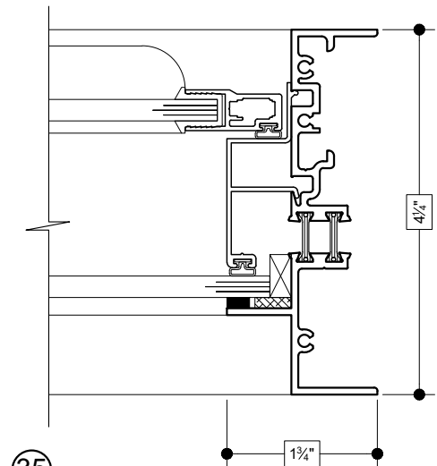
35 RIGHT JAMB (FIXED)
