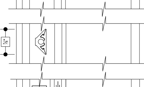
14 INTERNAL MUNTIN (TRAPEZOIDAL)
