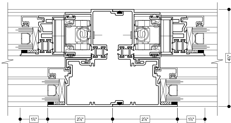
5 SELF-MULLION (SINGLE HUNG TO SINGLE HUNG)
