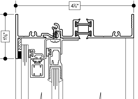
13 HEAD (SINGLE HUNG)
