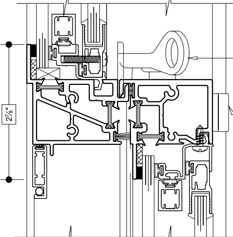
15 MEETING RAIL (SINGLE HUNG)
