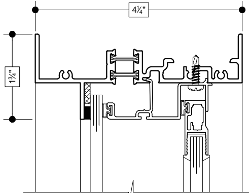
(27) HEAD (FIXED)
