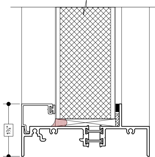
(30) SELF-STACK (OPERABLE OVER FIXED PANEL)
