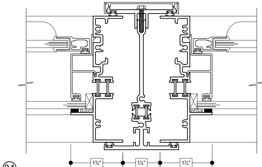
34 3-PIECE MULLION (FIXED TO FIXED)
