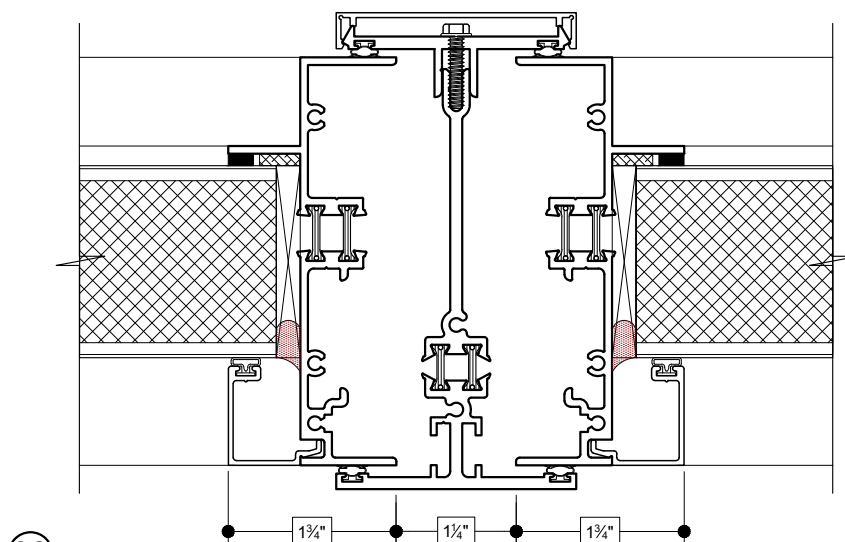
36 3-PIECE MULLION (FIXED PANEL TO FIXED PANEL)
