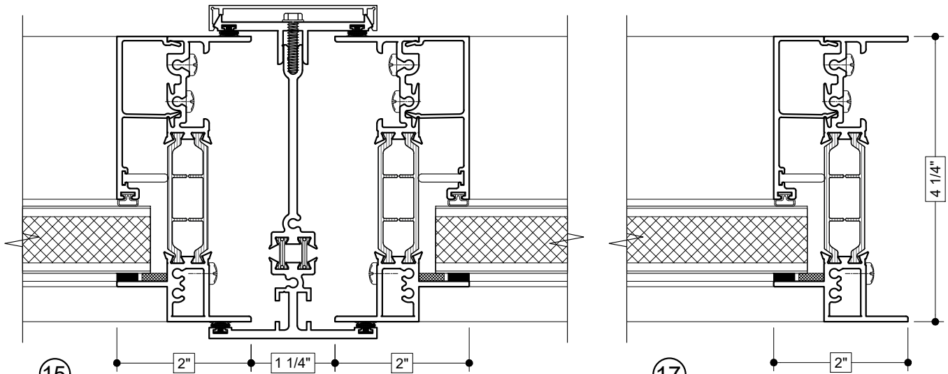
15 3-PIECE MULLION (FIXED PANEL TO FIXED PANEL)
