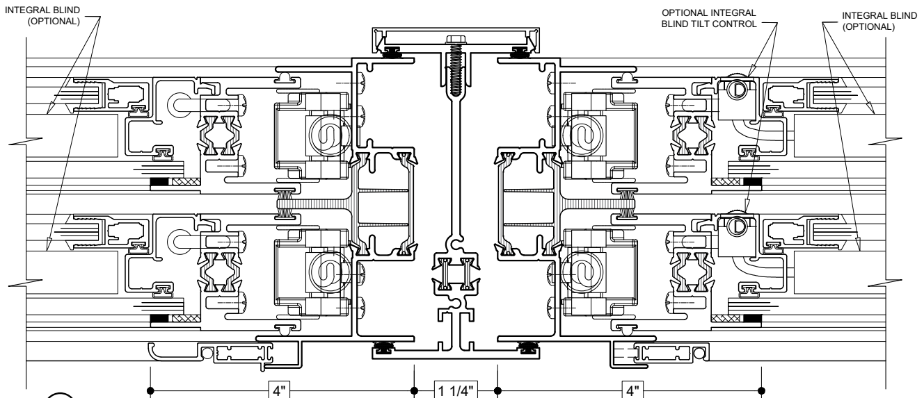
16 3-PIECE MULLION (DOUBLE HUNG TO DOUBLE HUNG)
