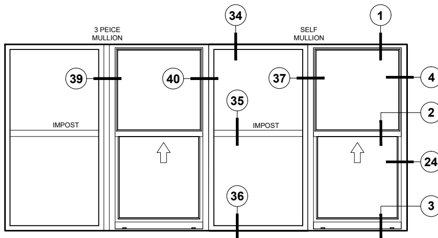
INSULATED GLASS SINGLE HUNG & FIXED LITES
