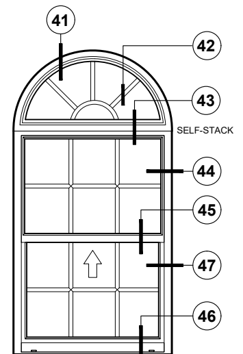
INSULATED GLASS EXTERIOR APPLIED TRAPEZOIDAL MUNTINS
