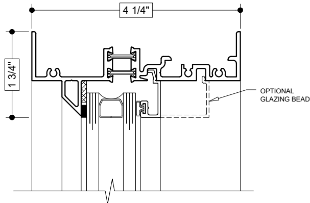
41 HEAD (FIXED)
