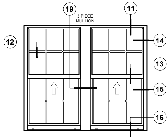
DUAL GLAZED INTERNAL COLONIAL MUNTINS
