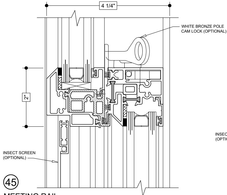
MEETING RAIL (SINGLE HUNG)
