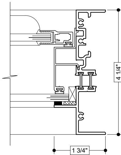
30 RIGHT JAMB (FIXED)
