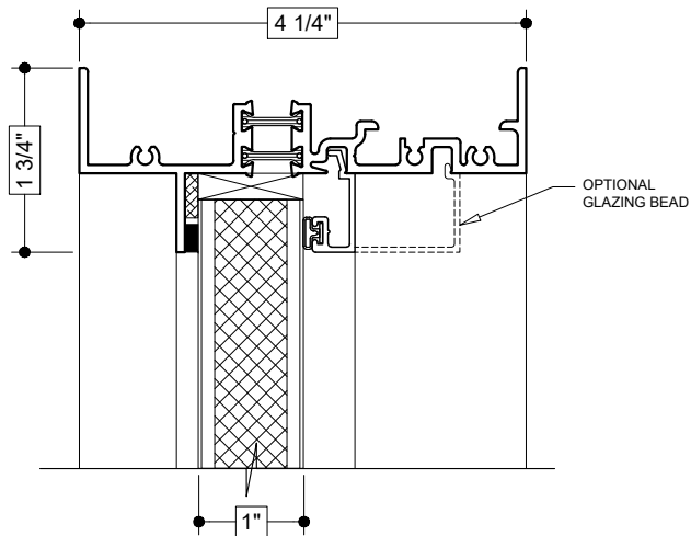
21 HEAD (FIXED PANEL)
