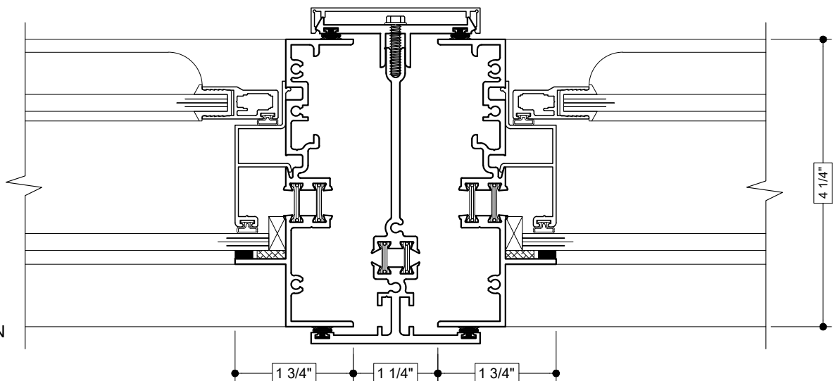
20 3-PIECE MULLION (FIXED TO FIXED)
