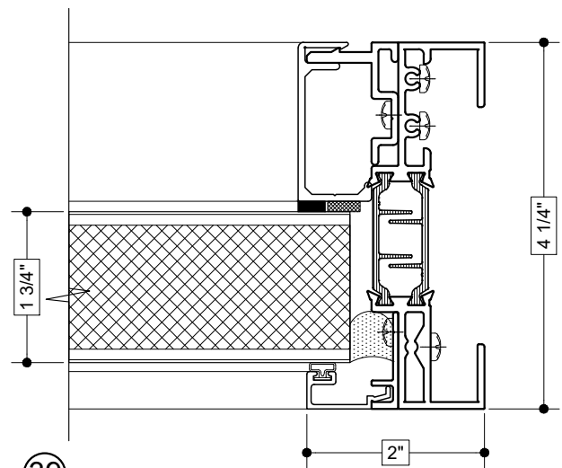
(39) JAMB (FIXED PANEL - UNIVERSAL)
