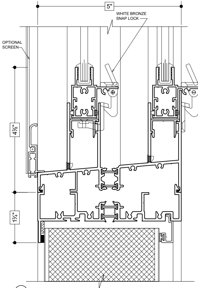
20 SELF-STACK (DOUBLE HUNG OVER FIXED PANEL)
