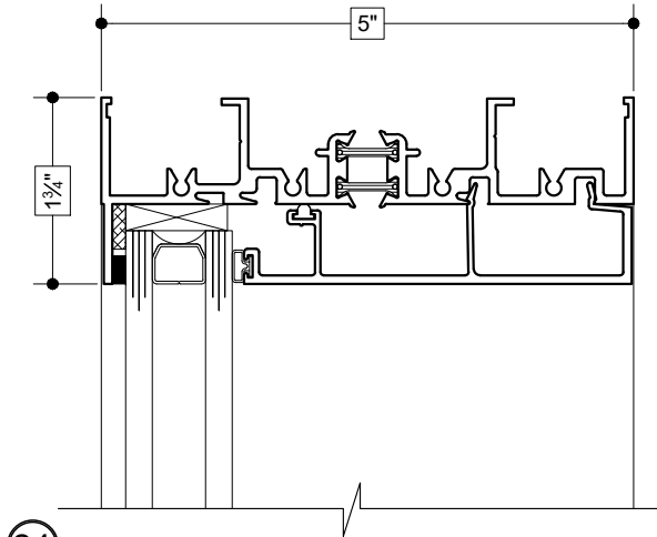
24 HEAD (FIXED)
