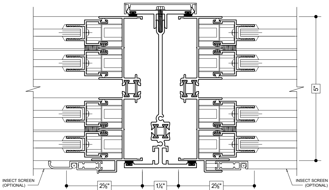
17 3-PIECE MULLION (DOUBLE HUNG TO DOUBLE HUNG)
