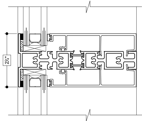
26 IMPOST (FIXED OVER FIXED)
