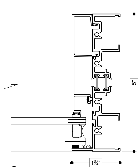
22 RIGHT JAMB (FIXED)
