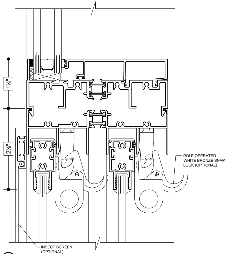
27 SILL (FIXED)
