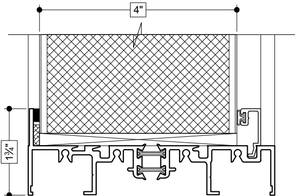
21 SILL (FIXED PANEL)
