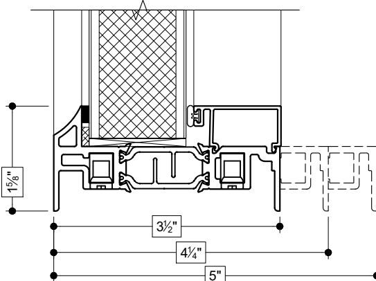
13 SILL (FIXED PANEL)
