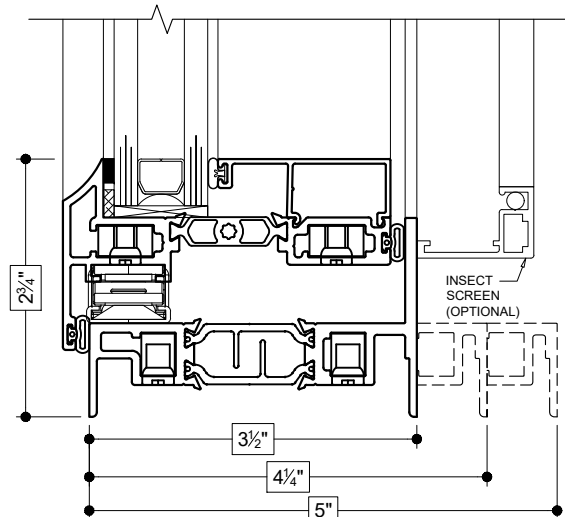
⑨ RIGHT JAMB (OUTSWING)
