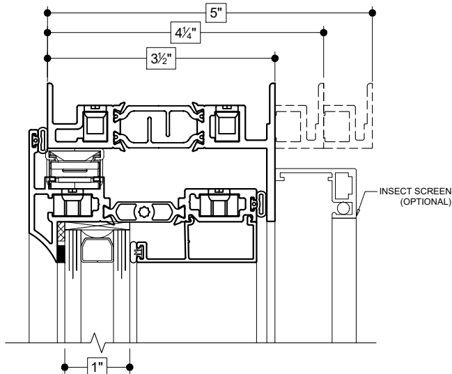
11 HEAD (OUTSWING)
