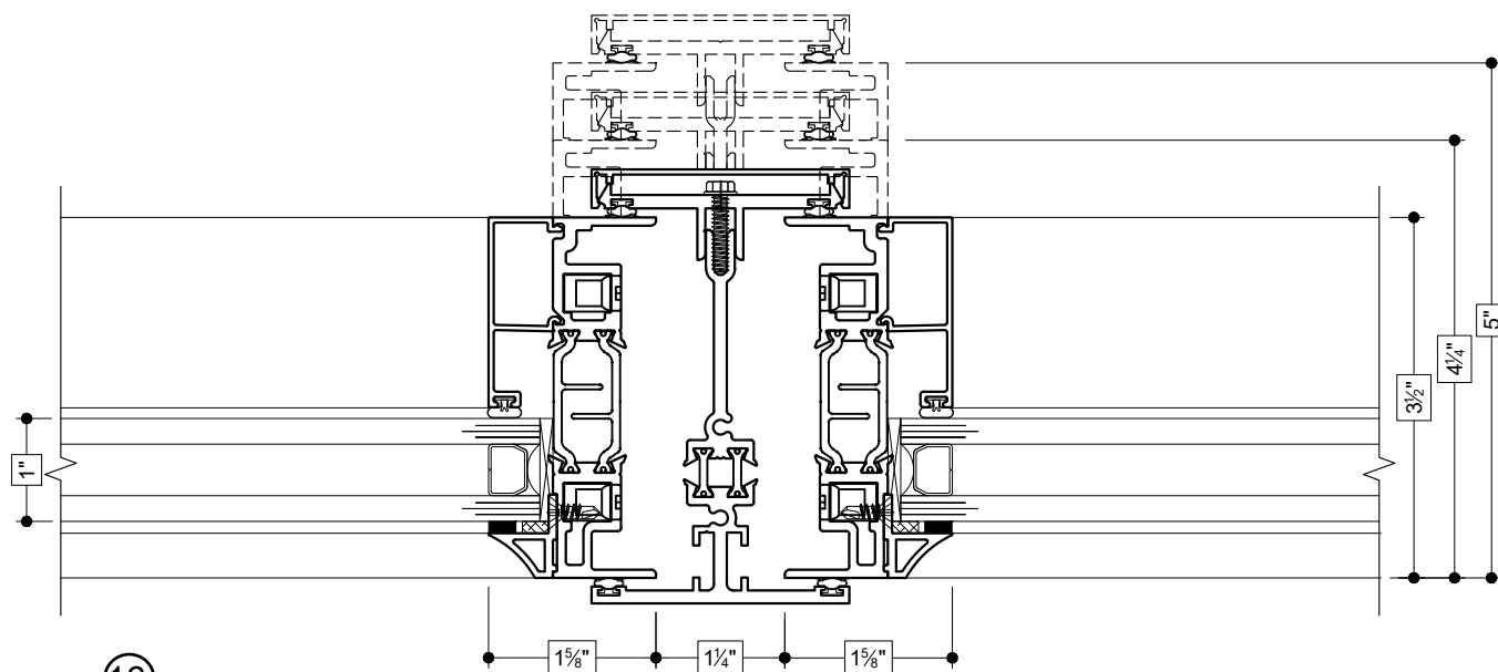
3-PIECE MULLION (FIXED TO FIXED)
