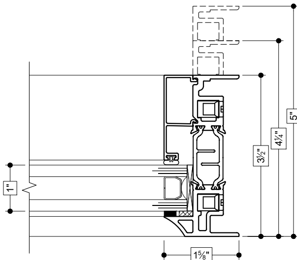
51 RIGHT JAMB (FIXED)
