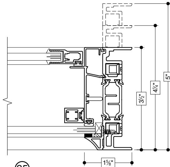
25 RIGHT JAMB (FIXED)
