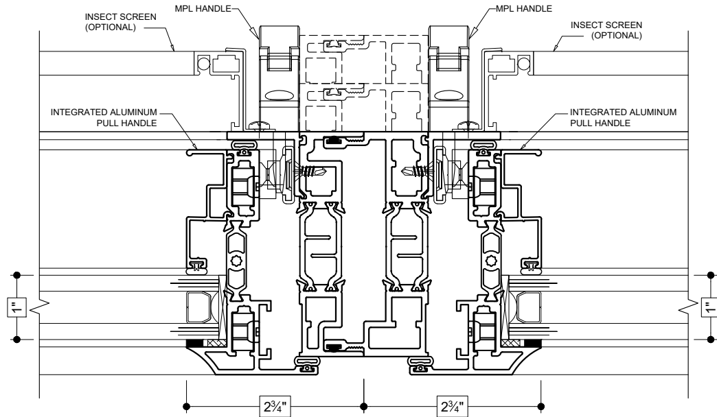
MALE/FEMALE JAMBS (OUTSWING TO OUTSWING)
