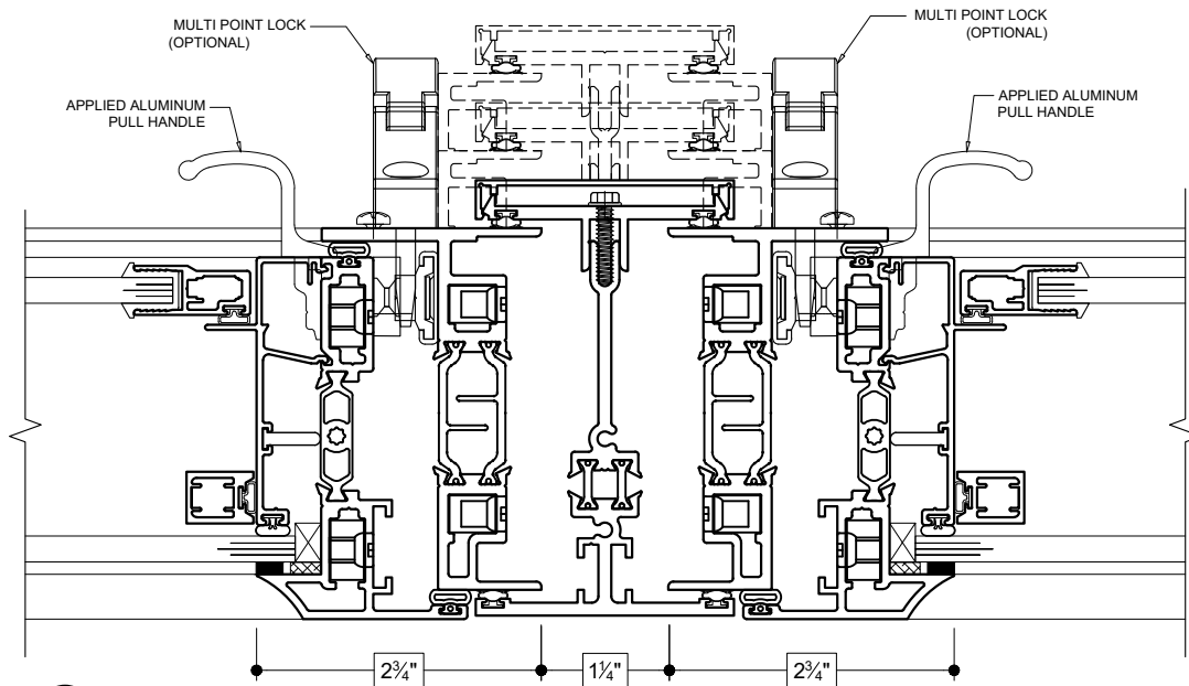
INTERNAL MULLION (OUTSWING TO OUTSWING)
