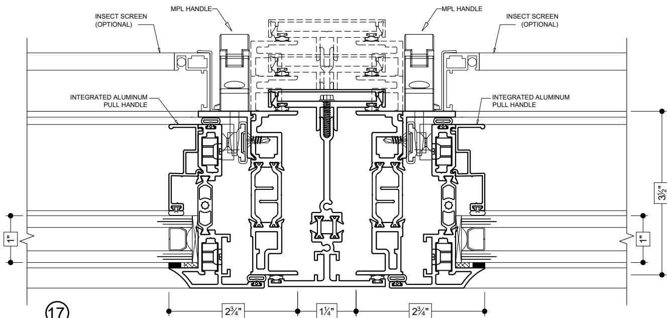
3-PIECE MULLION (OUTSWING TO OUTSWING)
