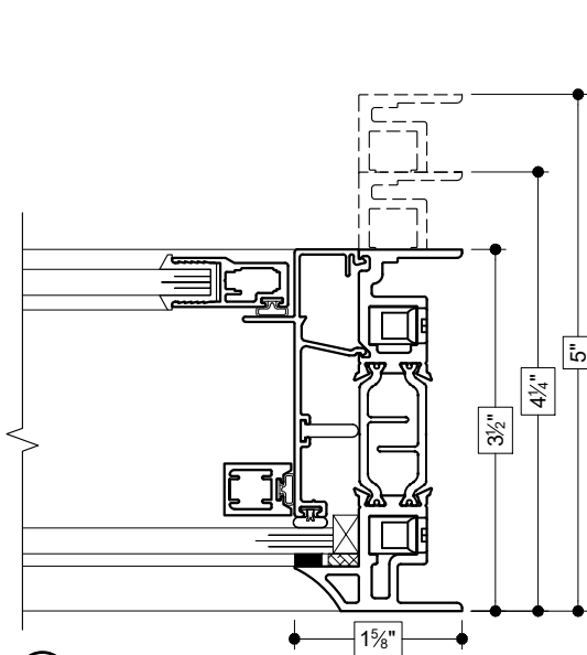
40 RIGHT JAMB (FIXED)
