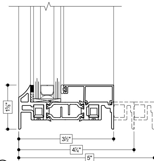
53 SILL (FIXED)
