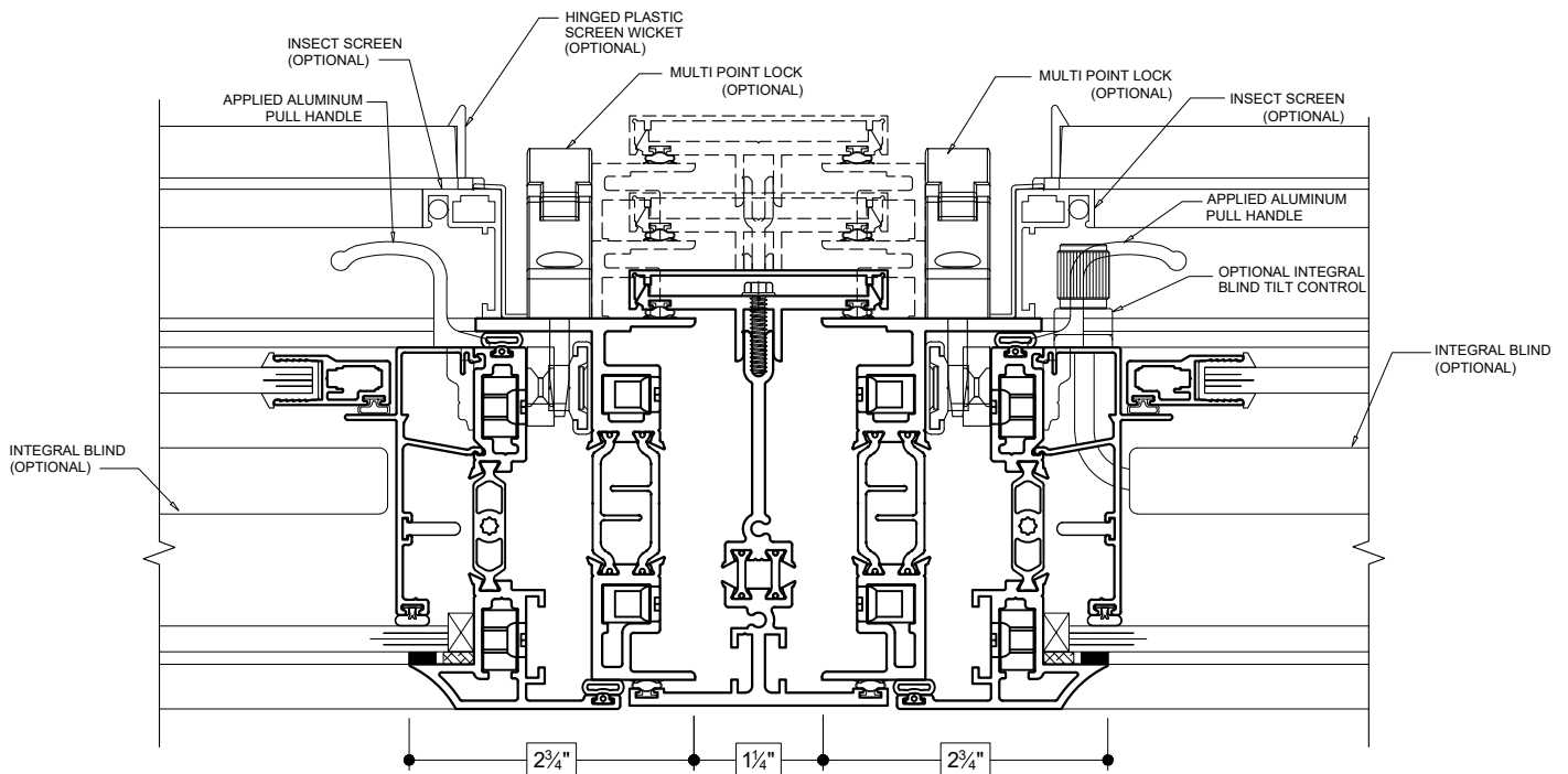
3-PIECE MULLION (OUTSWING TO OUTSWING)
