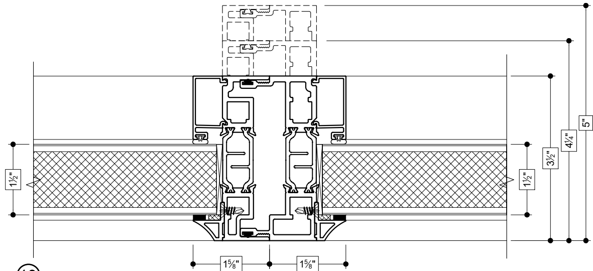
MALE/FEMALE JAMBS (FIXED PANEL TO FIXED PANEL)
