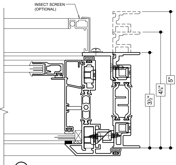
65 RIGHT JAMB (OUTSWING)
