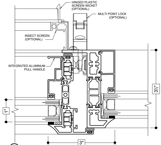
52 IMPOST (PROJECT-OUT TO FIXED)
