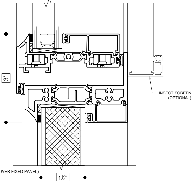
12 IMPOST (PROJECT-OUT OVER FIXED PANEL)
