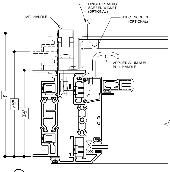
63 LEFT JAMB (OUTSWING)
