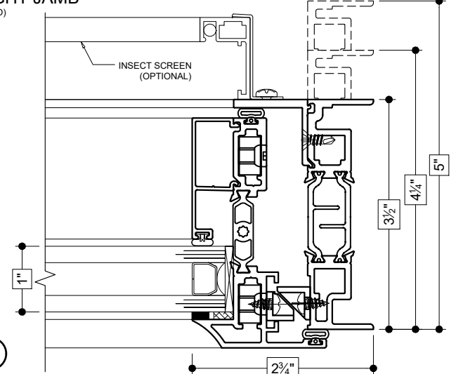
⑧ RIGHT JAMB (FIXED)
