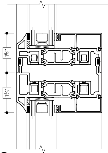
62 STACK-MULLION (FIXED OVER OUTSWING)
