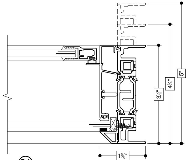
64 RIGHT JAMB (FIXED)
