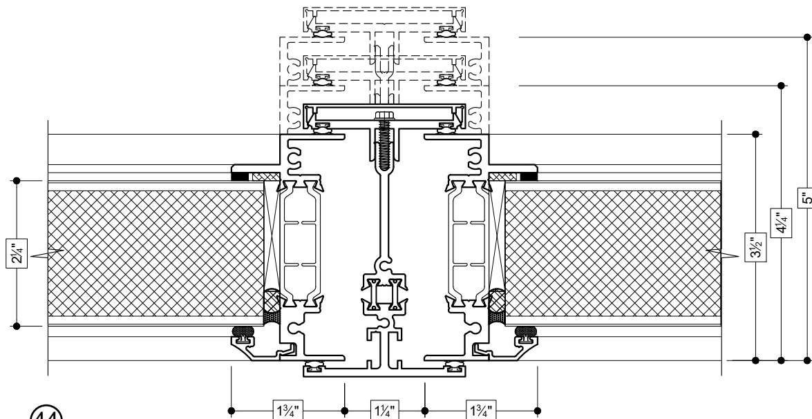
INTERNAL MULLION (FIXED PANEL TO FIXED PANEL)
