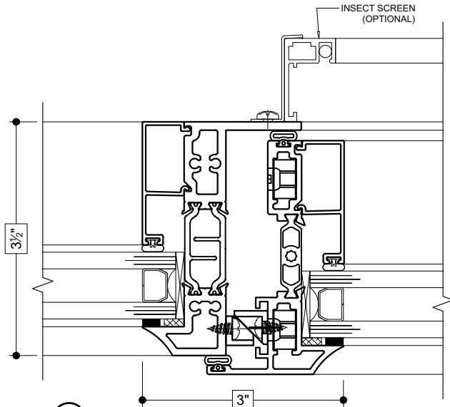
50 IMPOST (FIXED TO PROJECT-OUT)
