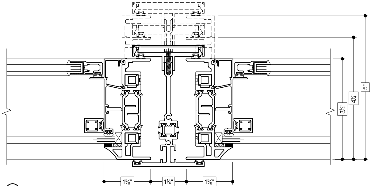
41 SELF-MULLION (FIXED TO FIXED)
