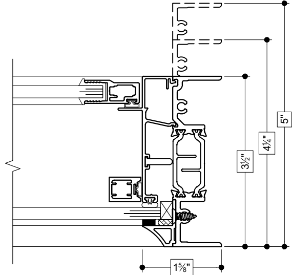
14 RIGHT JAMB (FIXED)
