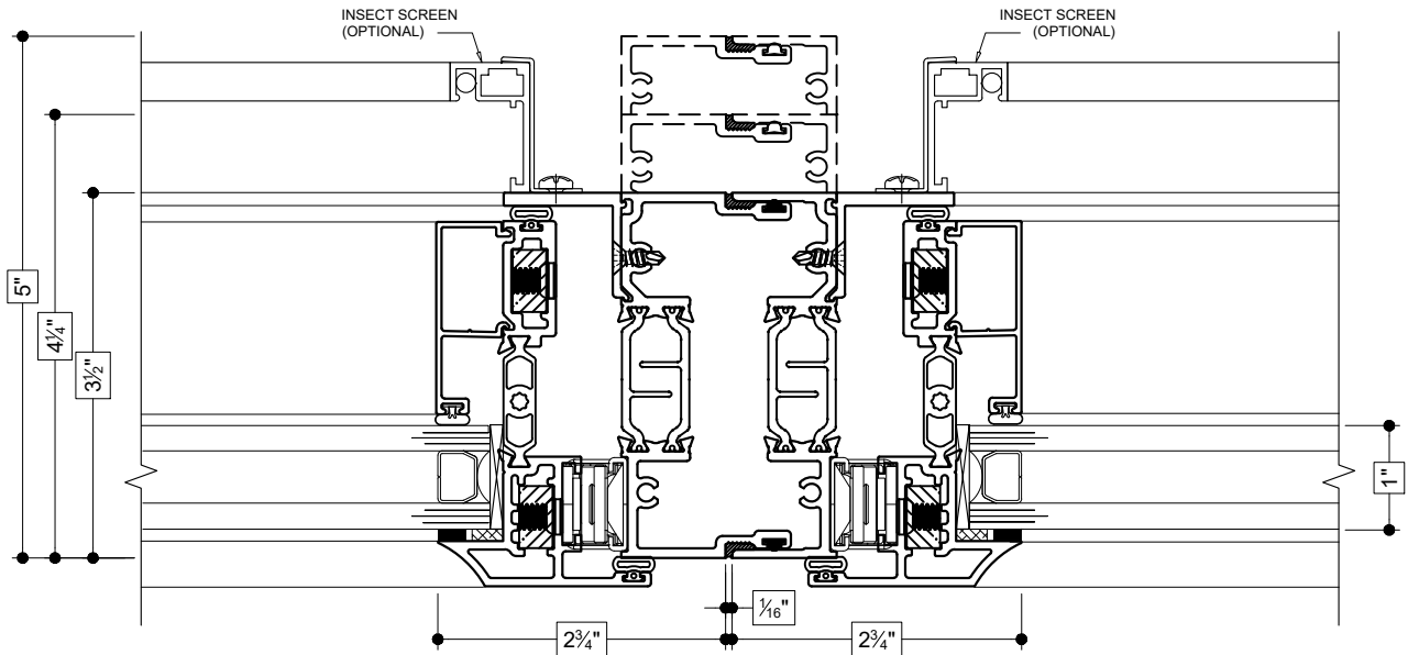
(21) SELF-MULLION (PROJECT-OUT TO PROJECT-OUT)
