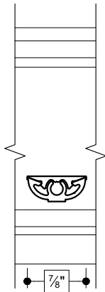
12 2-PIECE INTERNAL MUNTIN (COLONIAL)
