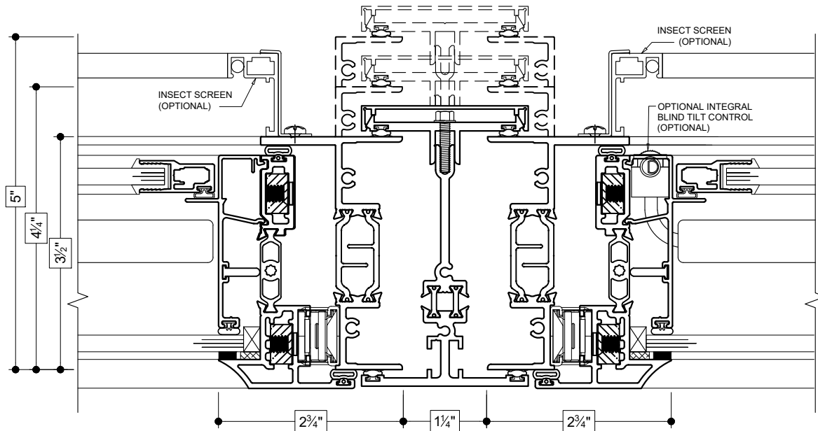
(28) 3-PIECE MULLION (PROJECT-OUT TO PROJECT-OUT)
