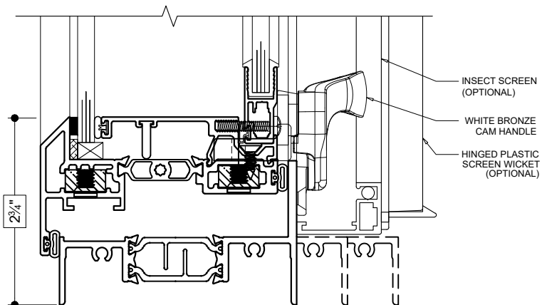
35 SILL (PROJECT-OUT)
