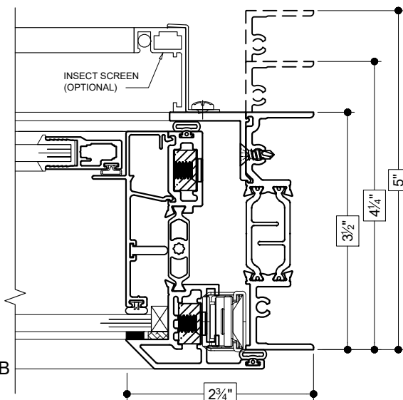
37 RIGHT JAMB (FIXED)
