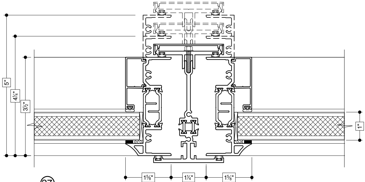
(27) 3-PIECE MULLION (FIXED PANEL TO FIXED PANEL)
