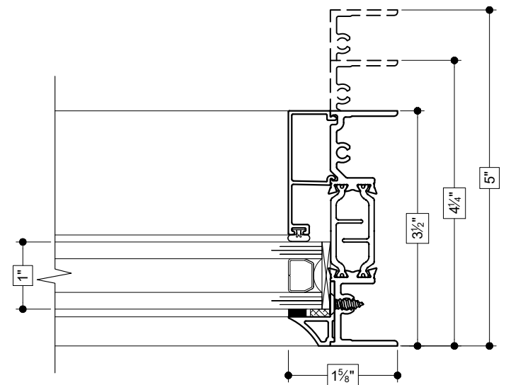
49 RIGHT JAMB (FIXED)
