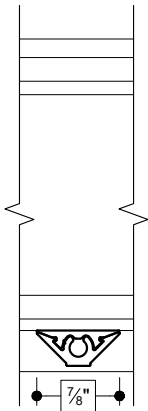
11 2-PIECE EXTERIOR MUNTIN (TRAPEZOIDAL)
