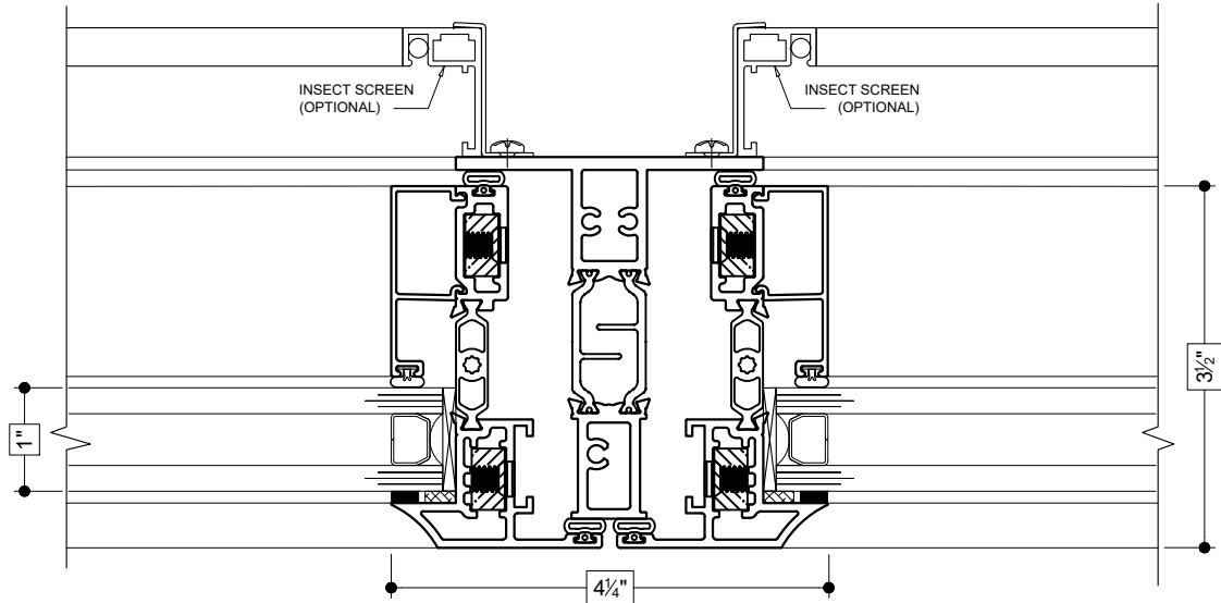
(50) IMPOST (PROJECT OUT TO PROJECT OUT)
