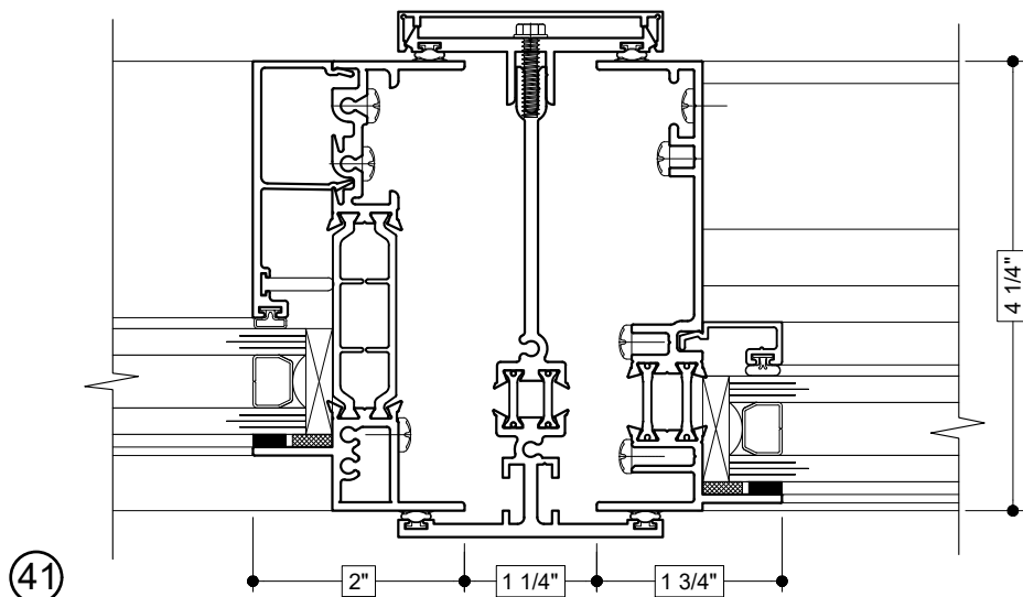
41 3-PIECE MULLION (FIXED TO SLIDER)
