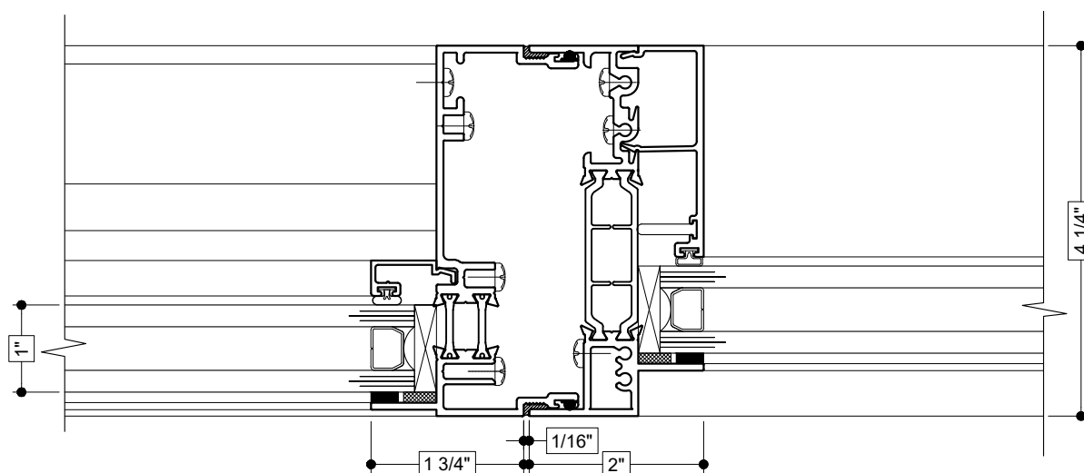
37 SELF-MULLION (FIXED TO FIXED - 7700i)
