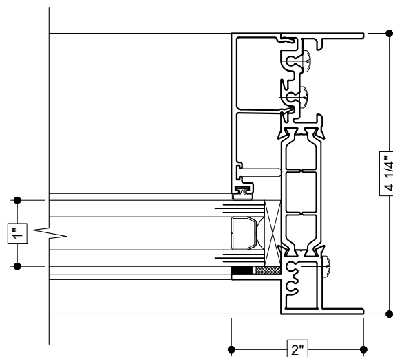
38 JAMB (FIXED) (SERIES: 7700i)
