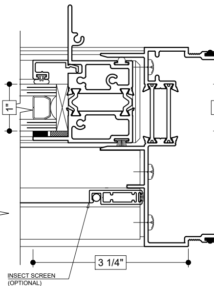
MALE FRAME
