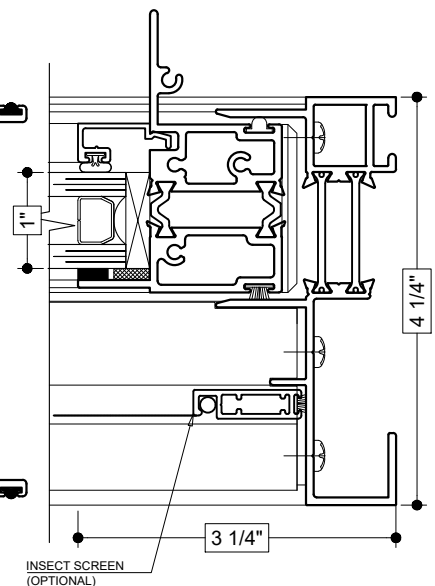
RETURN LEG FRAME
