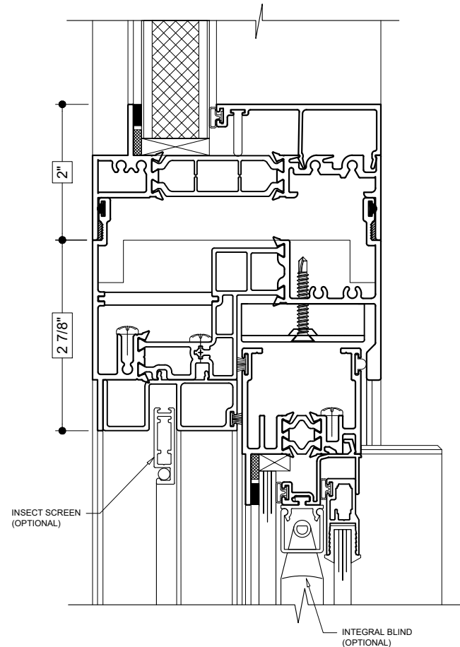
23 SELF-STACK (FIXED PANEL OVER OPERABLE)
