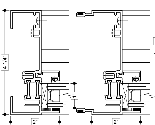
RETURN LEG FRAME
