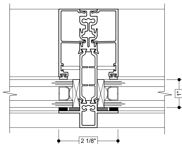
36 IMPOST (SERIES: 7700i)
