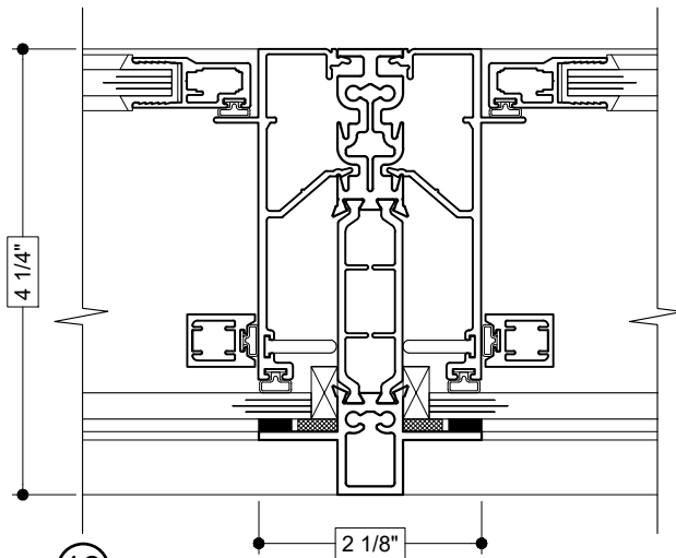
18 IMPOST (SERIES: 7700i)
